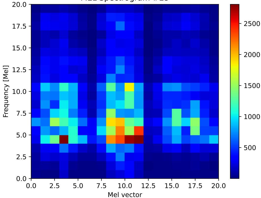
MEL Spectrogram #25
